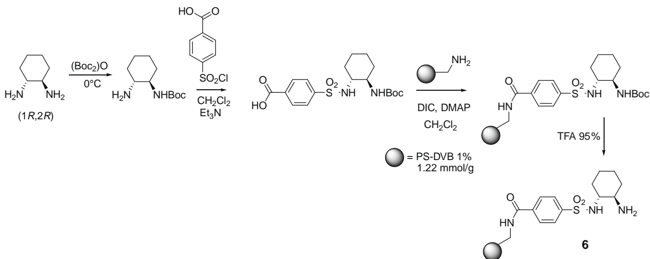
Scheme 1. Synthesis of the immobilized ligand 6 .
