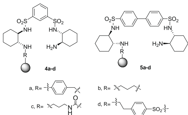
Figure 1. Supported ligands derived from ligands 1 and 2.
